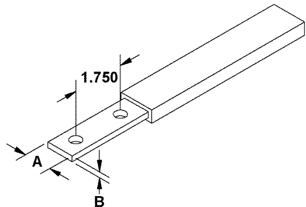
HOLE PATTERN "A"
